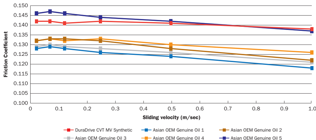
DuraDrive CVT MV Synthetic has high and stable metal-to-metal friction providing reliable power transmission.
