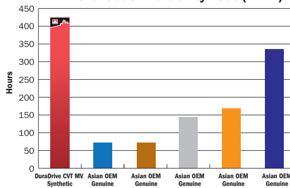
DuraDrive CVT MV Synthetic shows superior performance with extended shudder control when compared to OEM Genuine CVT fluids.
